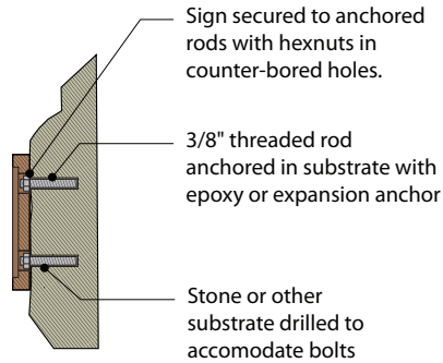
Section, Mounting Detail 2
