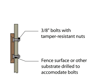
Section, Mounting Detail 1
